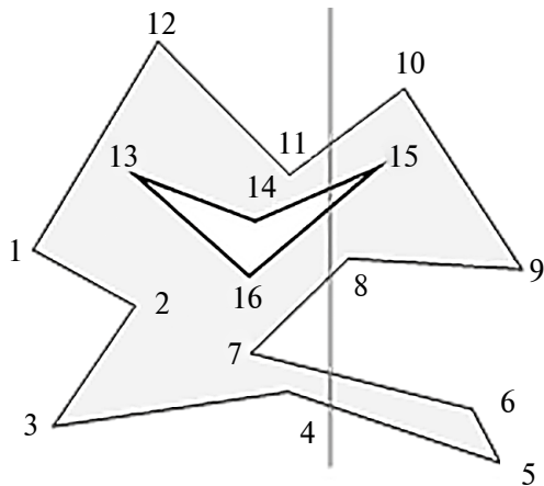
Рис. 3. Монотонные ветви границы фигуры: 1–12–11–10–9, 7–6–5, 7–8–9, 3–4–5, 1–2, 3–2, 13–14–15, 13–16–15.
