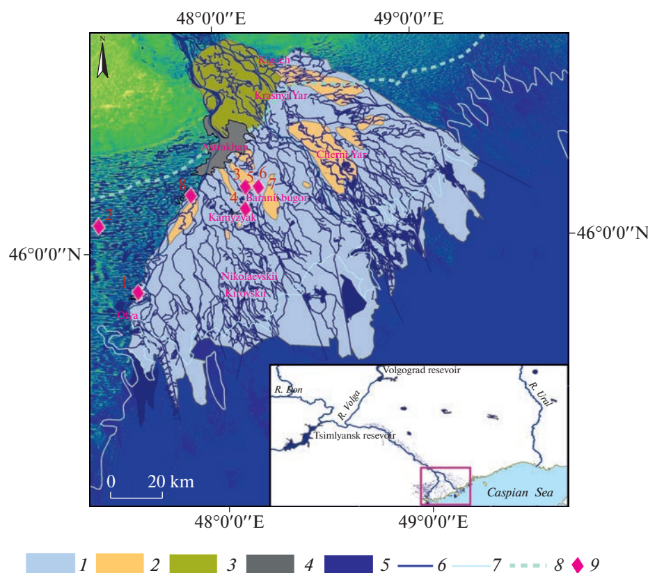
Fig. 1. Geological sketch and geographical setting of the Volga Delta: 1 – Holocene alluvial-marine deposits ( Q_{4am} ); 2 – Late Pleistocene alluvial-marine outliers ( Q_{3am} ); 3 – Volga floodplain ( Q_{4a} ); 4 – Settlements; 5 – Ilmeni and broad river deltaic channels; 6 – Rivers and channels; 7 – Coastline; 8 – New Caspian marine boundary ( Q_{4m} ); 9 – work area.
